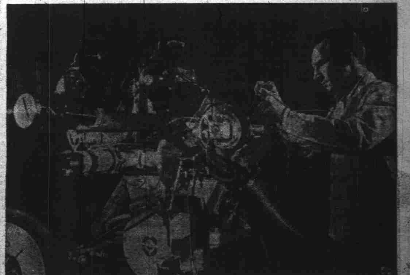
TEST FOR FORD MOTOR —To determine the power output which can be expected from 12 cylinders, above two-cylinder model of the aviation motor Henry Ford hopes to adapt to mass production is undergoing tests (above) at Detroit. After a study of many aircraft motors, Ford engineers now have in the making a 12-cylinder, V-type, liquid-cooled motor with injectors.
