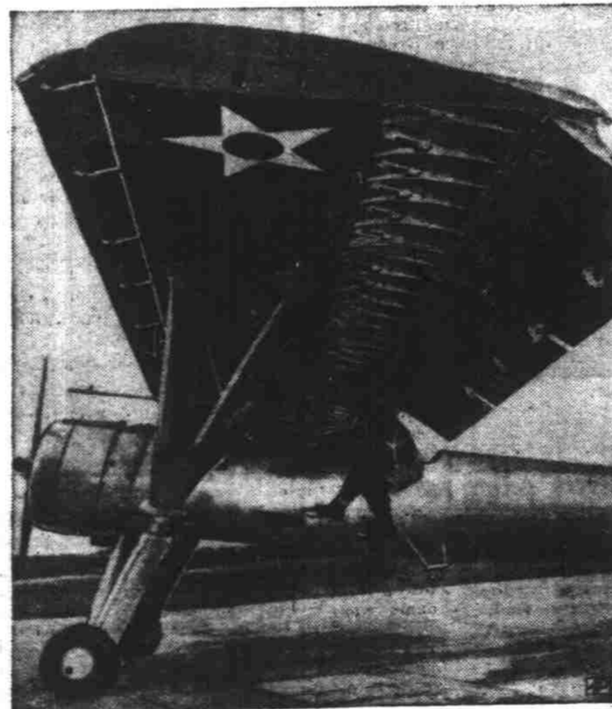
ARMY 'JEEP' —Pilots testing this plane at Fort Benning, Ga., call it the "Jeep." Wing slots on the leading edge and wide flaps on the trailing edge allow for quick takeoffs and landings at 25 m.p.h. Plane may serve as a courier.
