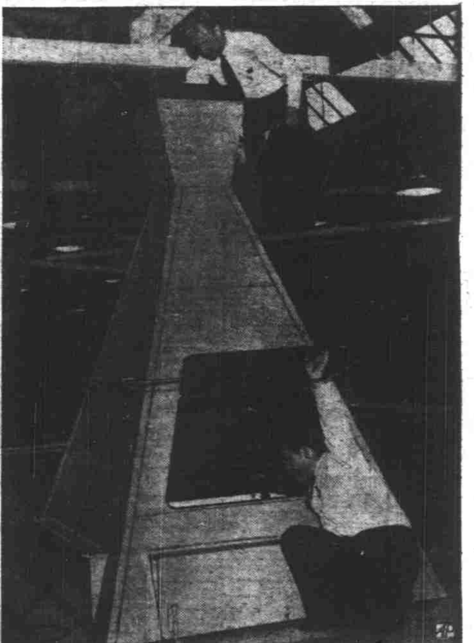
CAMERAS SPEED PLANE WORK —To cut down time interval between engineering on a new model plane and its initial flight two giant cameras are used in the Lockheed aircraft plant at Burbank, Cal. They make patterns for sections and parts under a new photo-left-template process. Camera stands 10 feet high, uses a 10-inch focal length lens and plates half a yard long.
