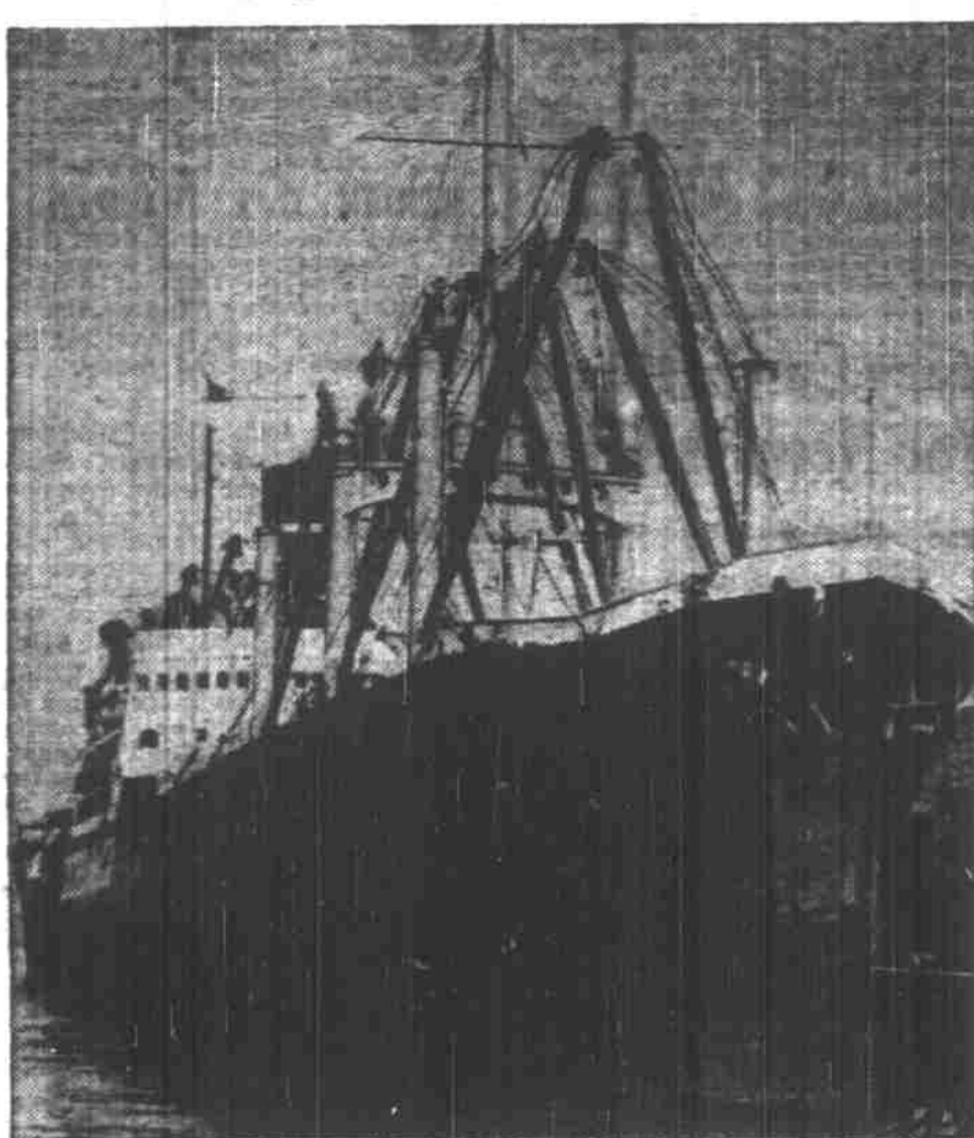
With a gaping 12 foot hole in her starboard bow, 20 feet above waterline as result of a collision with the Norwegian motorship Panama Express in a fog 170 miles north of San Francisco, the steamer Walter Luckenbach limped back to San Francisco safely.
