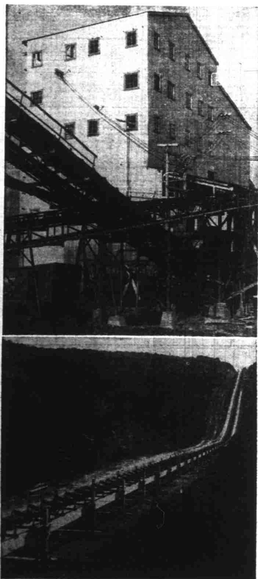
Manufacture of the 5,000,000 cubic yards of concrete to be placed in northern California's Shasta dam will require more than ten million tons of sand and gravel, called aggregate, which is washed and screened in a six-story mill, shown above, constructed especially for the task. Raw stock is excavated from a river deposit near Redding, Calif., will be transported on a ten-mile system of belt conveyors, section of which is shown below creeping across a hill. Belt line crosses the Sacramento river twice, crosses railroad tracks, five county roads, four creeks. Dam will be a major link in the vast Central Valley project.—HIN photo.
