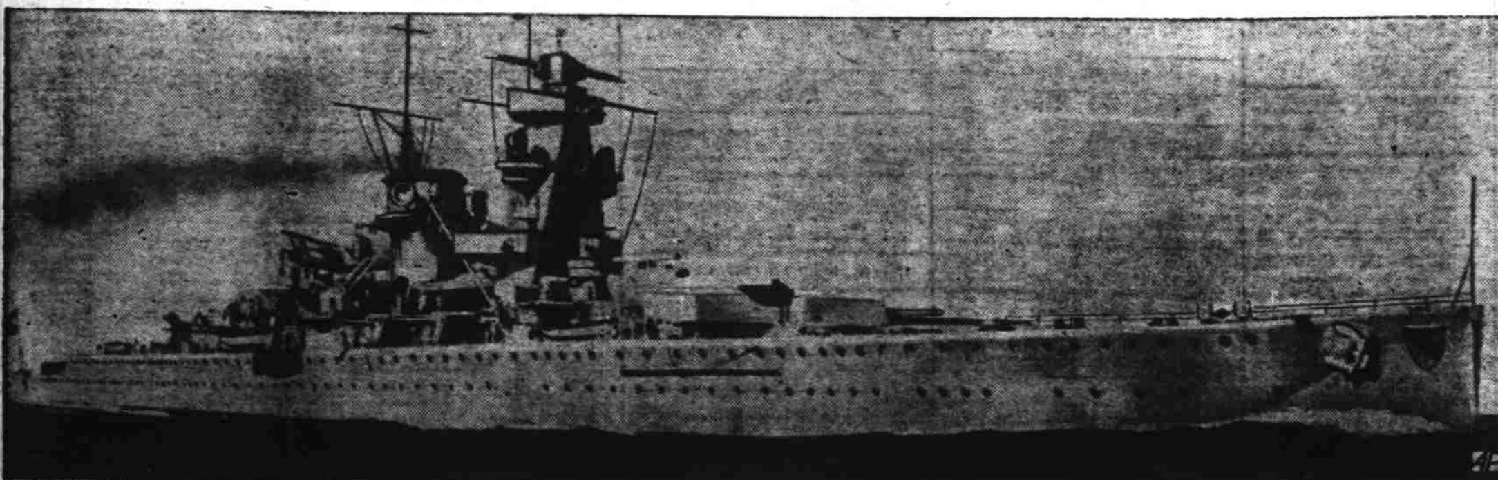
NAZIS POINT WITH PRIDE TO 'ADMIRAL SCHEER' —Reportedly the successful vessel which sank a British freighter, Clement, off Brazil, above 10,000-ton Admiral Scheer is one of three pocket battleships in Germany's navy; others are the Deutschland and the Admiral Graf Spee. These ships carry heavy armament consisting of six 11-inch guns, eight 6-inch guns, six large and three small anti-aircraft guns, and eight torpedo tubes. They also carry two seaplanes with catapults for launching. Clement survivors reaching Bahia, Brazil, reportedly identified the Admiral Scheer as Nazi boat which sank their freighter.
