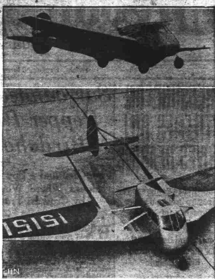
Heralded as a "foolproof" plane, this ship, two views of which are shown above, has been ordered by the federal government for the department of commerce. The plane, its designers say, can be flown easily by anyone who can drive an automobile. It can land in a steep glide, making it possible to clear high obstacles and get into a small plot of ground. Test flights were made at Ypsilanti, Mich.
