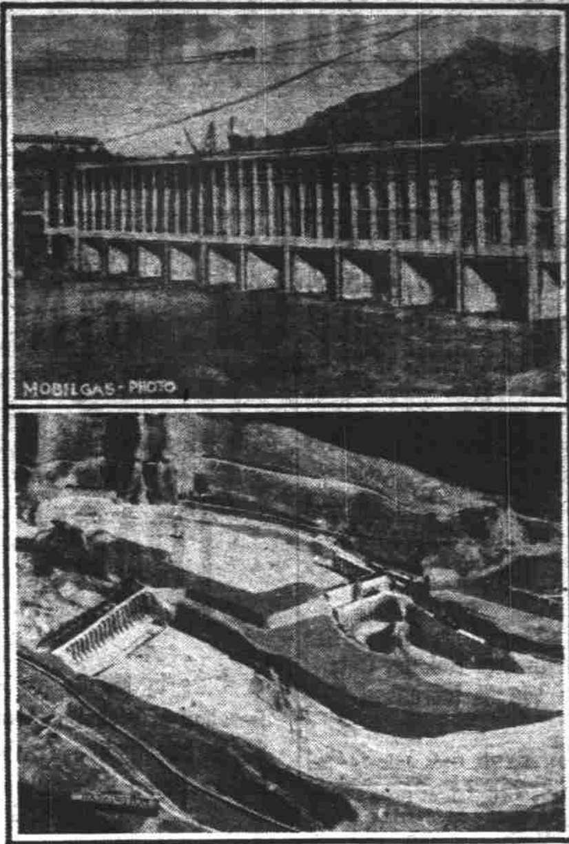
The huge Bonneville dam is rapidly taking form, as shown by the top picture of the sub-structure of the power house, obtained recently by the Mobilgas scout car. In the background is one of the mountains of the Cascade range on the Oregon side of the Columbia. Below is a picture of a model of the dam as it will appear when completed. The upper shore is Oregon and the lower shore Washington with Bradford Island in the center. Visitors are admitted to the project on Sundays only, according to the General Petroleum reporter.
