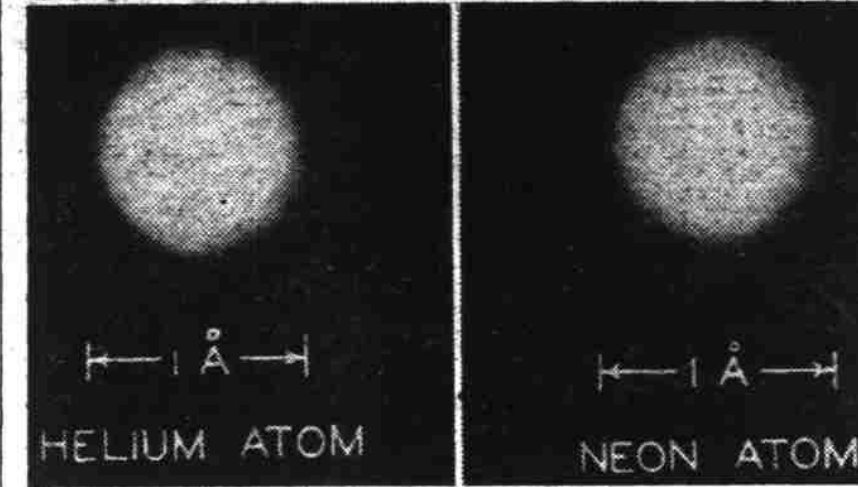
Here you see the first photographs ever made of the atom, magnified 200,000,000 times. They were made by Dr. E. O. Wollan (left) and Dr. Arthur Compton, of the University of Chicago, with a special microscope in which X-rays were used instead of ordinary light. Photos were shown at National Academy of Sciences in Washington.
