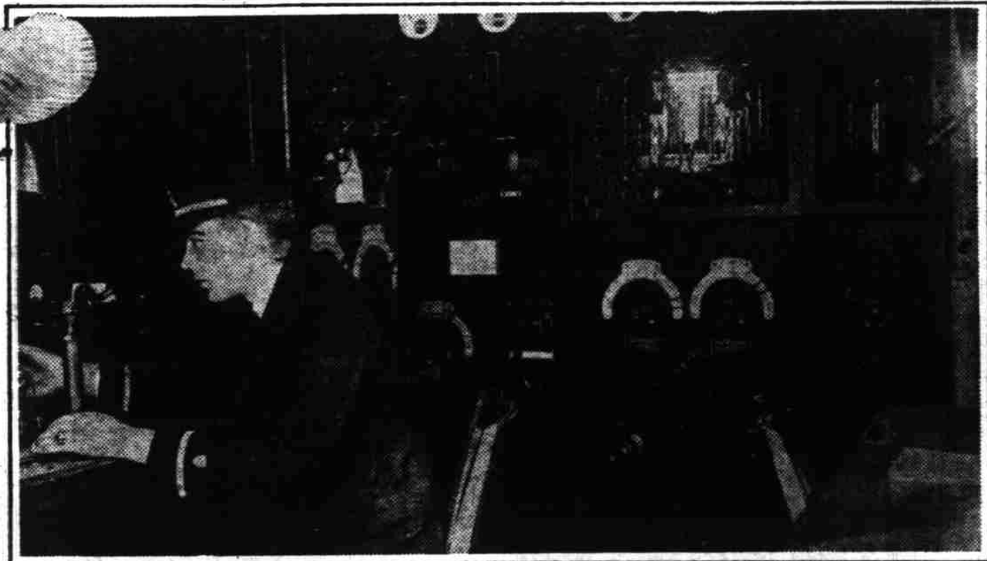
UNCLE SAM'S NEWEST CUTTER has three transmitters and three receiving sets in its radio room, shown above. It is the U. S. coast guard cutter Chelan, snapped at Washington, and cost $1,000,000. Ensign L. B. Tollaaksen is in the photo.
