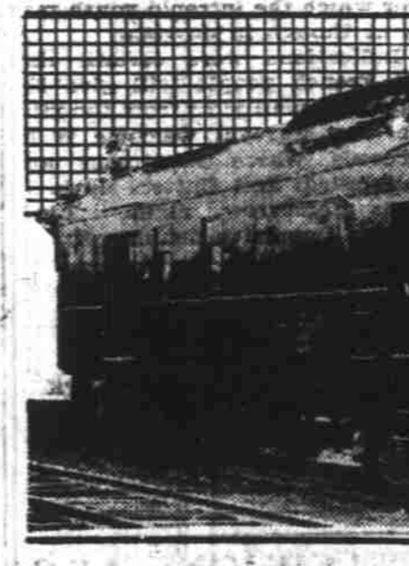
The photo, taken in St. Louis, Mo., shows one of a fleet of six gas-electric railroad locomotives being used to replace the steam locomotives on a western railroad.
