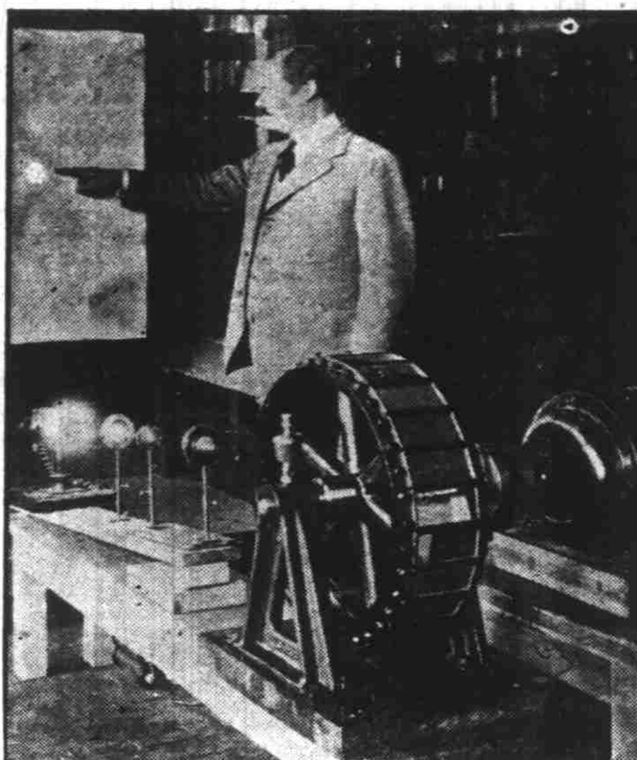
Cluster of seven lights used in television projector by means of which Dr. E. F. W. Alexanderson, consulting engineer of the General Electric company and the Radio Corporation of America, expects to reproduce moving objects by radio. When the drum covered with mirrors is revolved at great speed the entire screen is covered with brilliant lights. Dr. Alexanderson and the machine are shown in photo.
