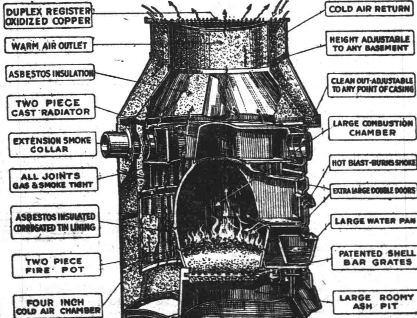
UNIVERSAL PIPELESS FURNACE
