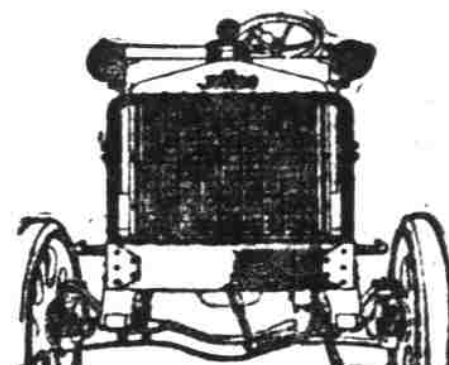
Motor-meter, Radiator Guard, Tow Hooks, Extended Frame forming Bumper, Radiator Shutters (closed) and Electric Lights.
