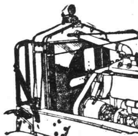
Radiator Fan Shroud forming perfect air tunnel so that entire surface of radiator is uniformly cooled.
