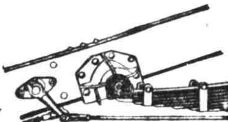
Front Rear Spring Bracket exceptionally strong. Top leaf wrapped full around eye for safety.
