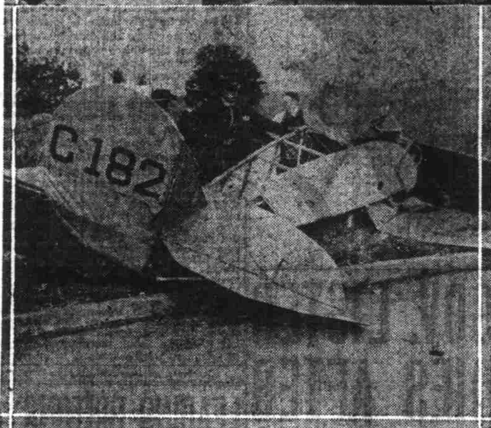
Wreckage at scene of disaster in which W. B. Hutchinson, late army aviator, and Sergeant John Milkowski, mechanic, were instantly killed after it had crashed nose down into cement walk opposite municipal golf links at Eastmoreland. Bottom—Tail structure of wrecked plane, supposed to have become jammed and prevented proper maneuvering.
