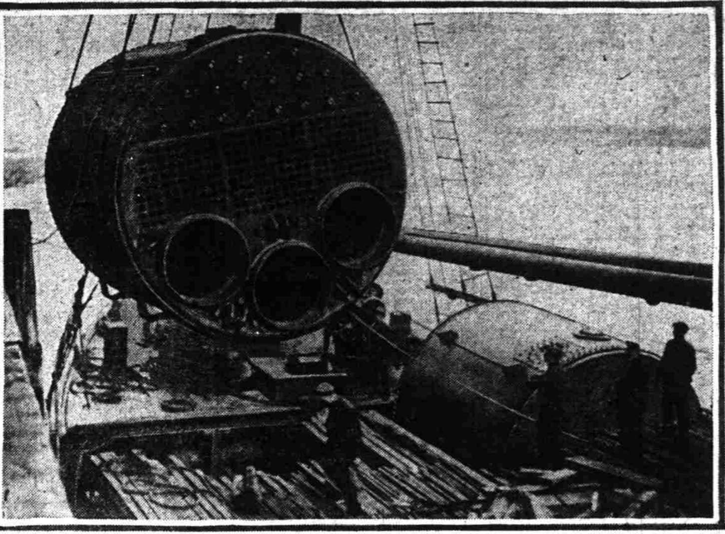
Weighting over 40 tons each, two big Scotch marine boilers for installation in the lighthouse tender Cedar were loaded on the steamer Bee, at the Willamette Iron & Steel Works, Monday, and today are on their way to San Pedro. The Cedar is a new vessel for service on this coast, designed and built by the California Shipbuilding Co. of Long Beach.
