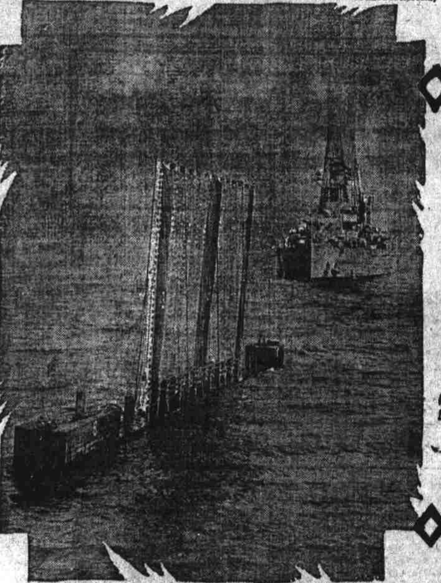
This is the Target, Only Twelve Feet High and Twenty-one Feet Wide, Which Was Struck Six Times in Fifty-seven Seconds by Six Shells Fired from a Single Twelve-inch Gun. The Remarkable Feature About This Feat Was That the Target Was Moving at the Rate of Five Knots and the Arkansas at the Rate of Ten Knots When the Shots Were Fired.
