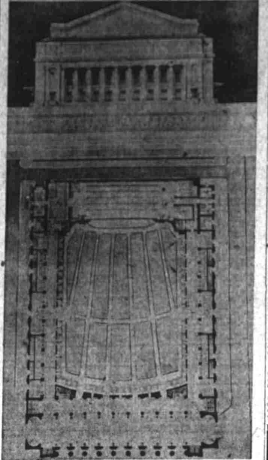
Front elevation of plan awarded first prize, and first floor design.
