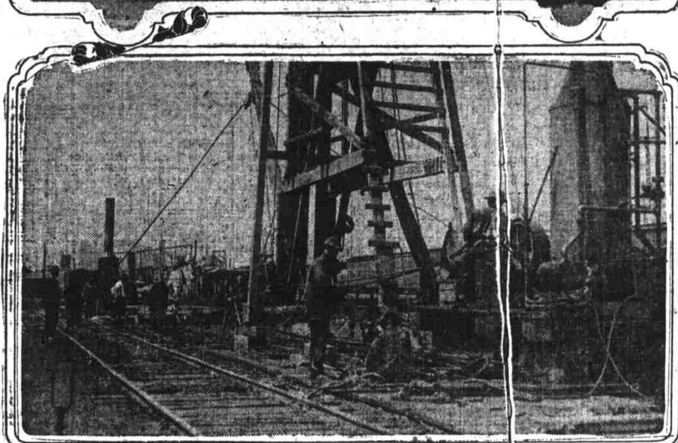
View from east side of river, showing piers on both sides and work on piers in middle of stream; workmen building Pier No. 2 in yards of Northern Pacific Terminal company.
