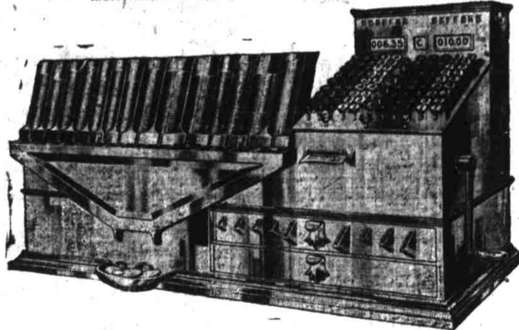
BILYEU AUTOMATIC CHANGE-COMPUTING MACHINE, for Department Stores and all classes of Retail Business. Both amount purchased and tendered will be visibly registered, stamped on sales slip, difference computed and paid as well as totaled. Now well into the metal and ready for demonstration in 60 to 90 days.
