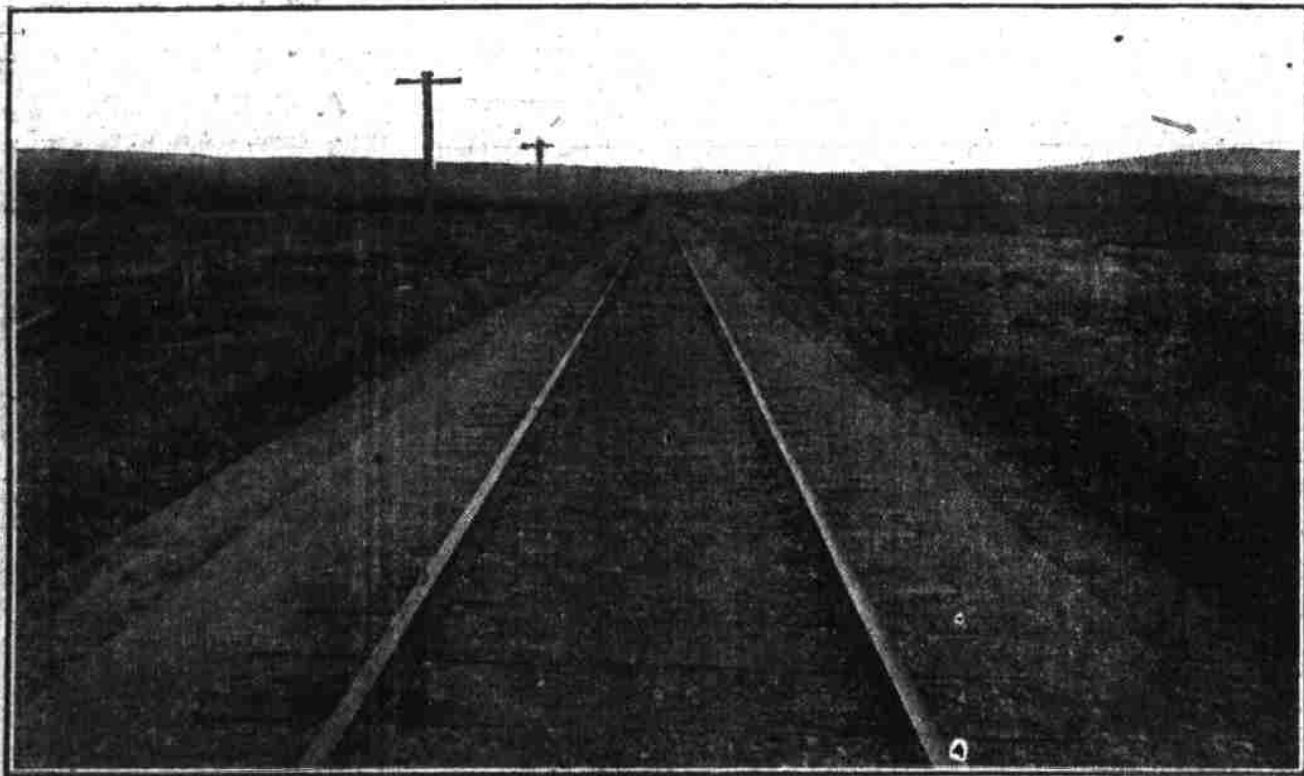
The picture shows a section of the O. R. & N. track across the Umatilla Reservation, ballasted with gravel from Umatilla. From Pendleton to Huron, on the summit of the Blue Mountains, the O. R. & N. roadbed, under the efficient General Roadmaster W. Bollons, has been placed in a condition rivaling the famous roadbed of the Pennsylvania, between New York and Washington. The work of improvement will proceed next year. General Roadmaster Bollons has had numerous bouquets from other railroad men for his good work in "maintenance of way," as the phraseology of the railroad world names it.
