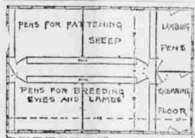
GROUND PLAN.
