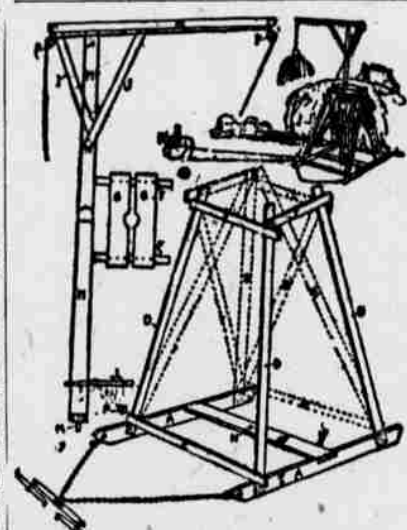
GOOD PORTABLE HAY DERRICK.
