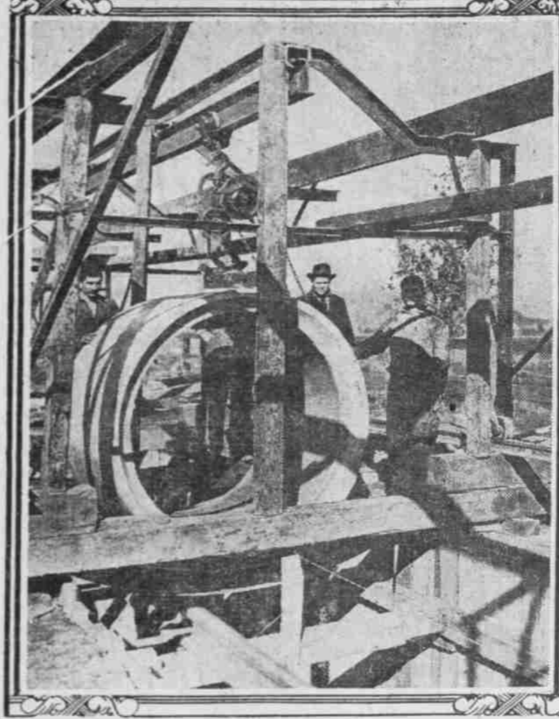
Lowering Section of New 5 Foot Trunk Sewer in Montavilla.
