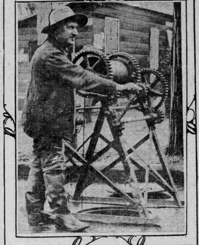
Upper—Nozzle" Attachment, Showing How the Water Is Thrown So as to Wash Out Sewer. Lower—Windlass Arrangement Which Drags Cleaning Machine Through Sewer at Rate of Ten Feet a Minute.
