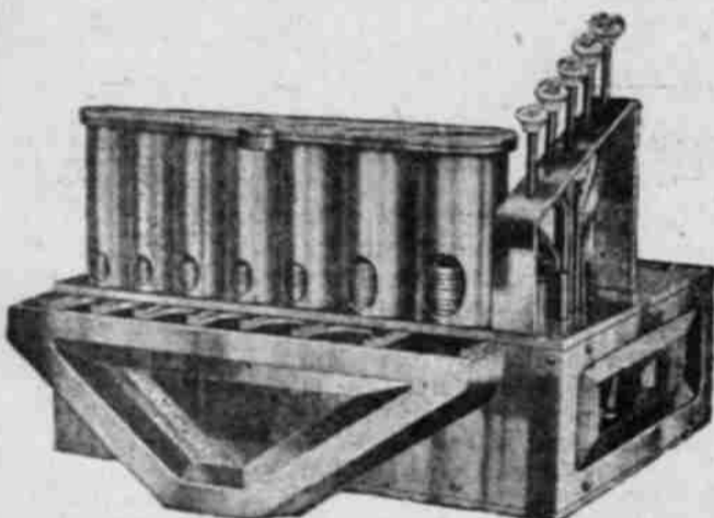
LIGHTNING CHANGE-MAKER For pay-as-you-enter streetcars, theaters and all other places where small change is handled extensively. Makes change instantaneously, for any amount up to $5.00, by pressing one key.
