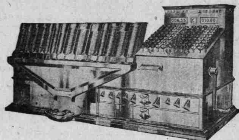
CHANGE-COMPUTING MACHINE For department stores and all classes of retail business. Visibly and permanently records amount tendered and amount of purchase, prints on sales slip, totals same and pays out correct change. Simplifies the balancing of cash. Prevents errors.
