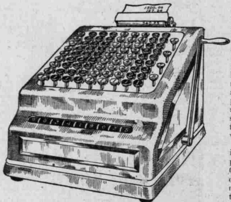
THE ADDING MACHINE Embodies all the good features of Adding Machines now on the market, and in addition is more flexible, with less parts.
