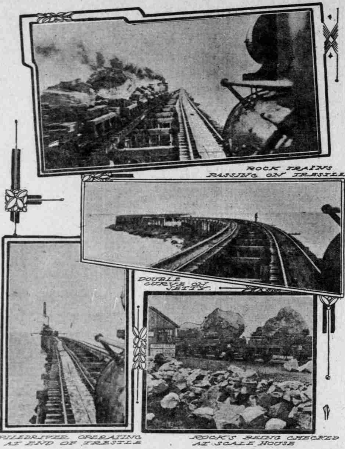
ROCK TRAINS PASSING ON TRASSIE. DOUBLE CURVE ON JETTY. PILEDRIVER OPERATING AT END OF TRESTLE. ROCKS BEING CHECKED AT SCALE HOUSE.
