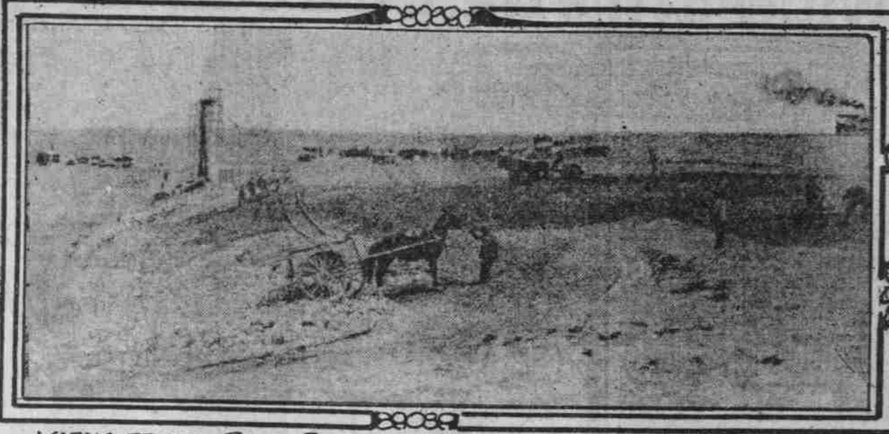
VIEW FROM COLD SPRINGS DAM. SHOWING TOWER WHERE WATER WILL BE TURNED ON AND OFF. DAM WHEN COMPLETED WILL BE SAME HEIGHT OF TOWER
