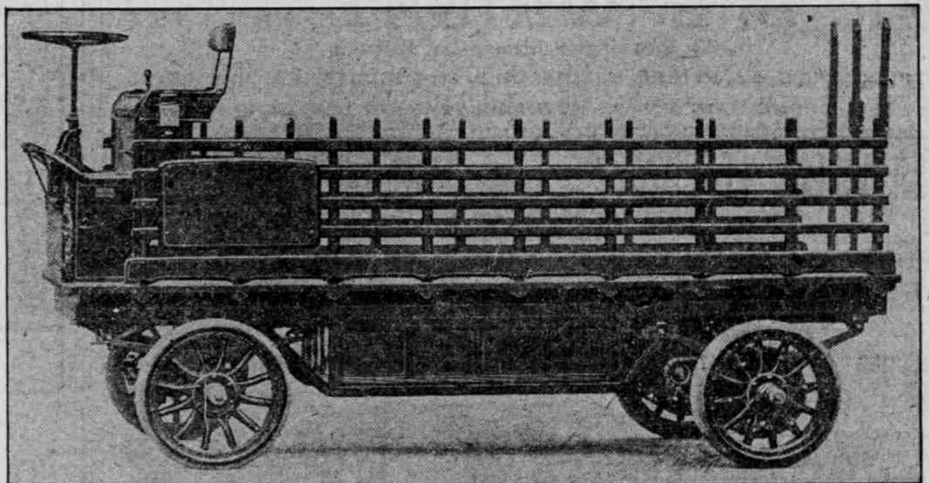
Studebaker Model No. 2012a Electric Truck
