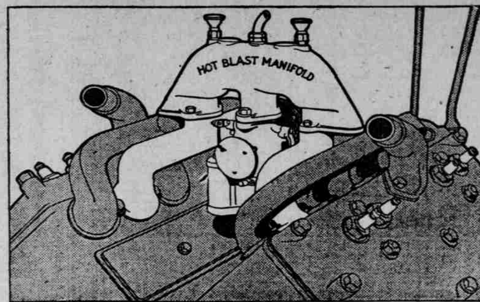
Aero-EIGHT Hot-Blast Manifold Assembly
