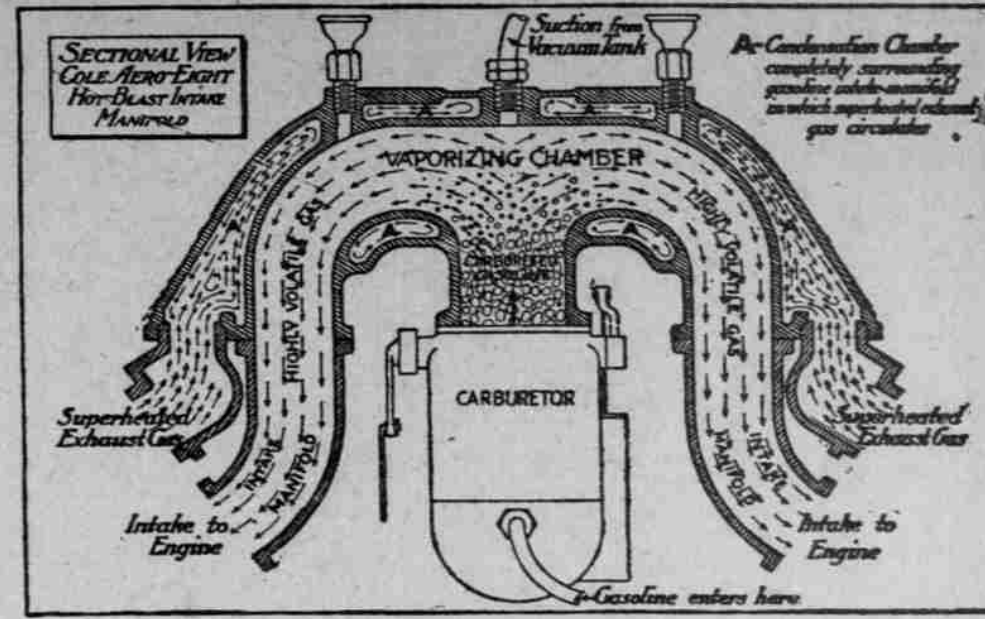
Operation of Aero-EIGHT Hot-Blast Manifold
