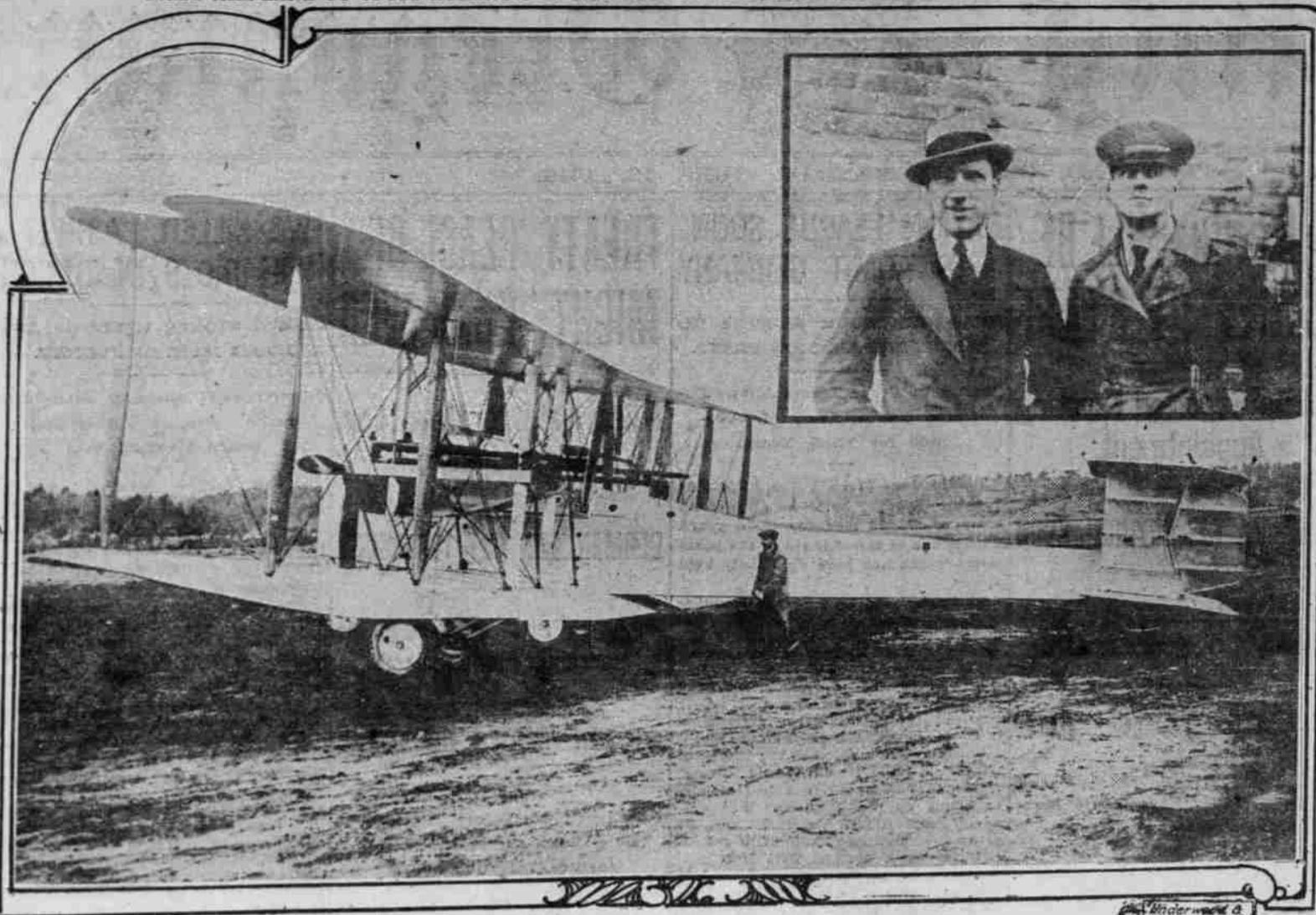
VICKERS-VIMY PLANE AS SHE APPEARED BEFORE START. INSERT, LEFT TO RIGHT, CAPTAIN JOHN ALCOCK, PILOT (BRITISH) AND LIEUTENANT ARTHUR W. BROWN, NAVIGATOR (AMERICAN).
