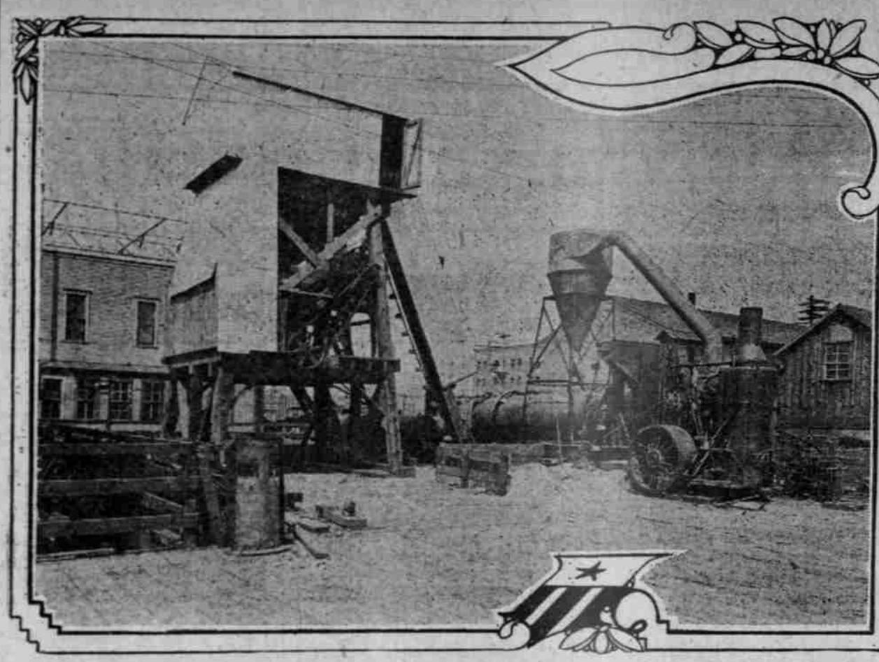
VIEW OF CITY'S NEW MUNICIPAL PAVING PLANT, WHICH HAS JUST BEEN COMPLETED.
