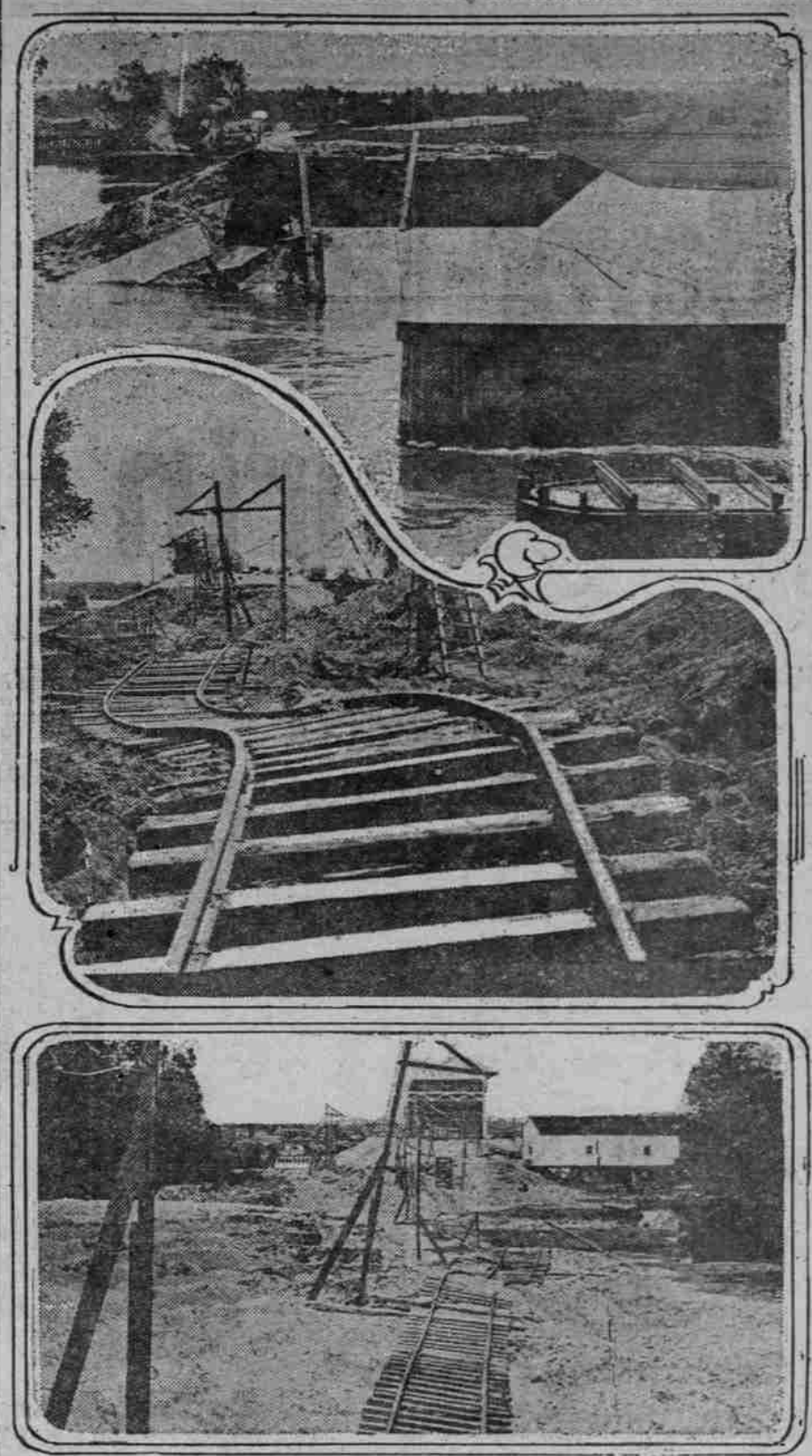
Top—Broken Concrete Work on South Side of Columbia Slough. Middle—Big Pier Which Dropped Almost to Water Level Suddenly When Three Men Were Walking Across It. Below—Showing Destruction of Hayden Island Between Truss Spans and Girder Spans.
