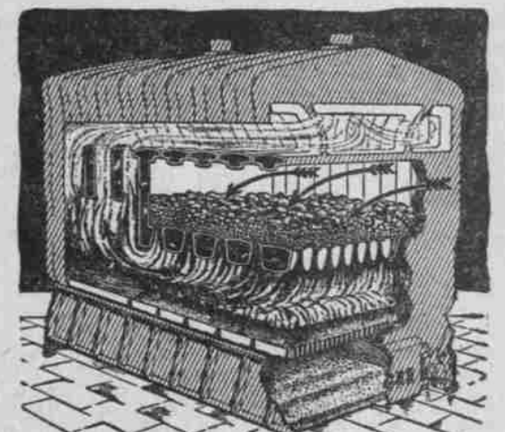
Open view of IDEAL Smokeless Down Draft Boiler to show by arrows how the air is made to pass down through the upper and lower grates or double fire to thoroughly mix with the flames and thus produce utmost heating results from cheapest soft coal, with Smokeless results. Big fuel capacity cuts down carting.
