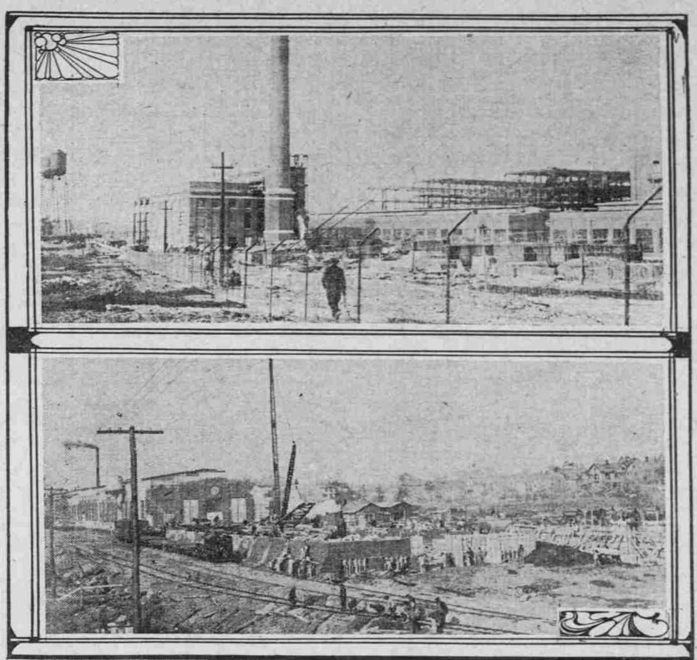
ABOVE—POWER PLANT AND BUILDINGS IN ITS VICINITY. BELOW—NORTH END OF WORKS.
