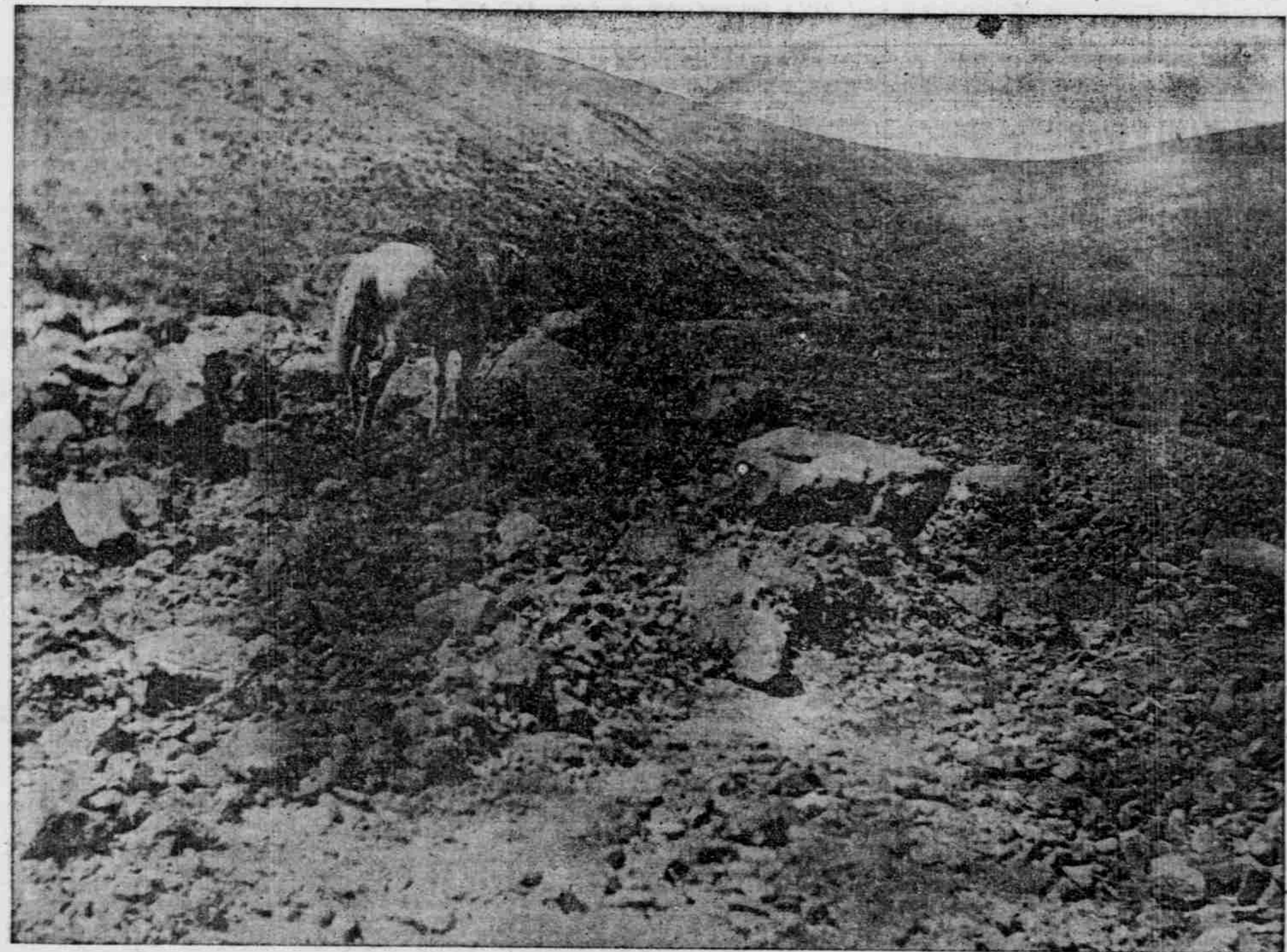
BOULDERS AND ROCK DEBRIS FROM A SMALL SIDE GULLY SIX MILES ABOVE HEPPNER.
