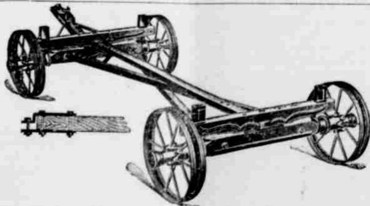
Straight or Cross Reach Orchard Trucks
