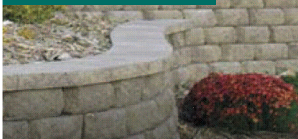
Diamond Gray Retaining Wall Blocks Build straight or curved retaining walls up to 4' tall. Nominal dimension 6" H x 15 7/8" W. X 12" D.
