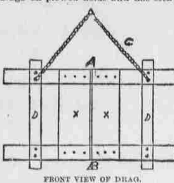
FRONT VIEW OF DRAG.
