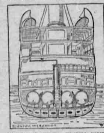
SECTION OF VESSEL SHOWING PORHYDROMETER.
