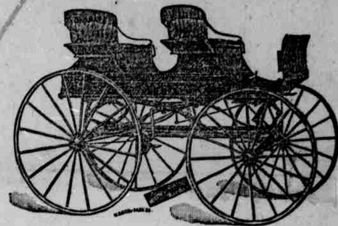
Four Spring or Mountain Wagon. We have them in three styles, plain, plain and cut away body. This is a very popular spring wagon, is built of the best second growth stock, the irons are hand forged Norway; double collar steel axles, "A" grade of wheels, steel tire, leather cushions, finely painted and finished throughout, and is the most handsome and suitable family spring wagon ever put upon the market. It is sure to please you and your family, and the time is now at hand when you can afford to own one, for our prices are down to bedrock.
