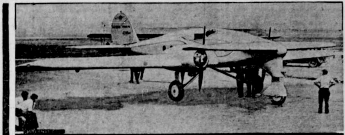
A view of the new and specially designed two-motored tandem monoplane which was tested at Roosevelt field, Long Island, in preparation for a proposed flight from New York to Bucharest, Rumania. The plane is said to be nonstallable, and a tricycle landing gear prevents noseovers.
