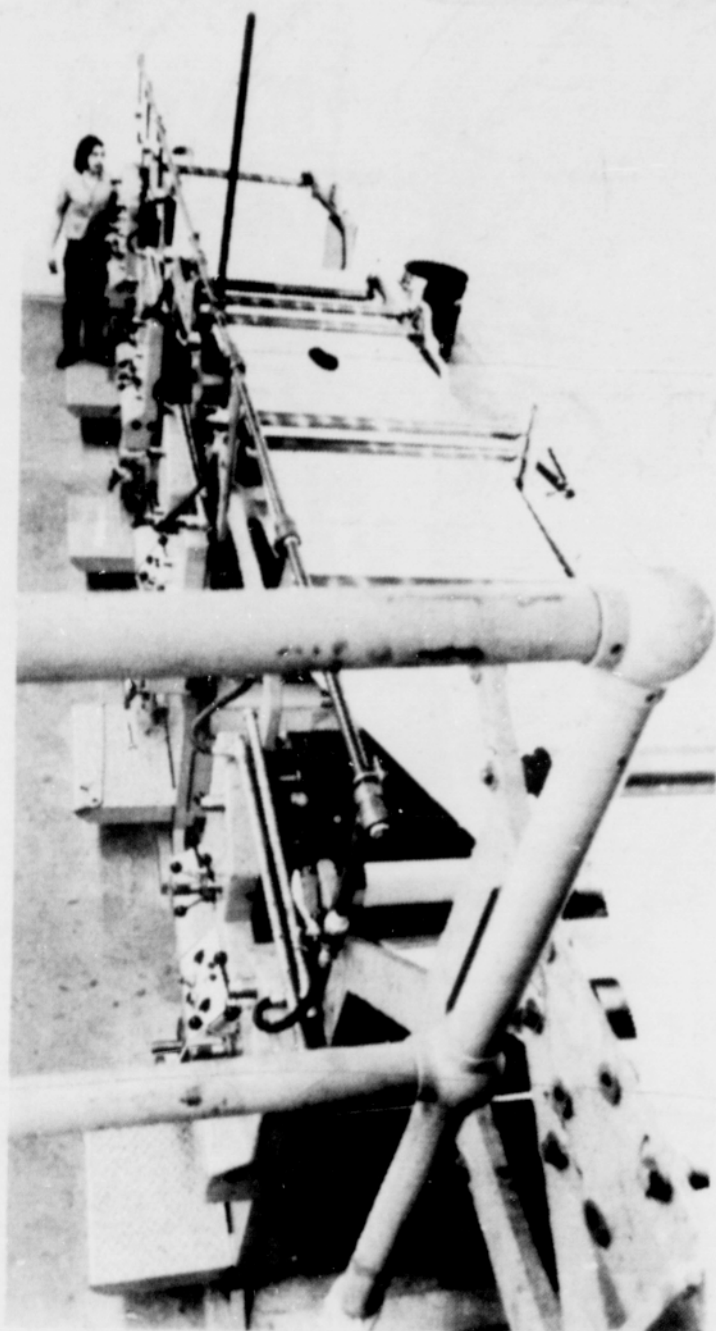
VIEW FROM UPPER DECK shows flow of paper as it moves in, under and over printing cylinders. (Outlook photo)
