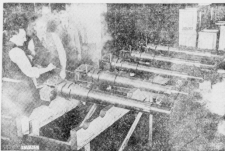
75 MM. howitzers for the U. S. army are shown being tested in an Erie, Pa., manufacturing plant. These guns will hurl a 14 lb. projectile a distance of 9,500 feet and are rated with the highest striking power of any army gun for its weight.
