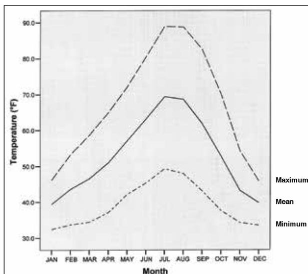
Figure 2. Monthly maximum, mean, and minimum temperatures for Grants Pass, Oregon 1889 - 2002.
