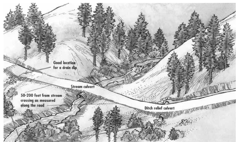
Ditch drainage should be directed into a vegetation filter, and not allowed to continue flowing down the ditch and into the stream.
