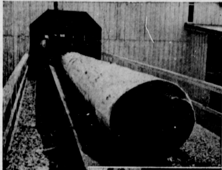
(Top) New look in sawlogs as barked Douglas fir enters mill on log haul. (Inset) Ring barker mechanism, showing two of four jets which flay off bark under water pressure of 1400 pounds per square inch.
