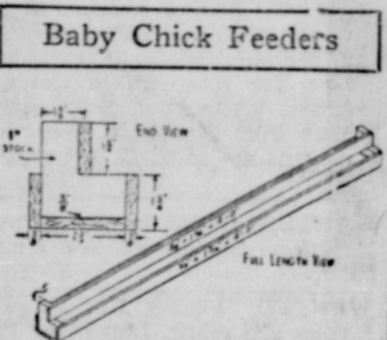
Baby Chick Feeders Preventing waste of feed is always important. Easily-built feeders of wood will help prevent waste of feed. This Washington State college design can be built at little cost. It will serve 100 chicks for their first 10 days.
