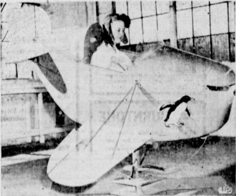
High school students will receive training in the fundamentals of flying if this motorized pre-flight trainer is adopted in the public schools. June Hamilton demonstrates the tiny trainer, showing that it can back, turn and pivot as well as the expensive trainers.
