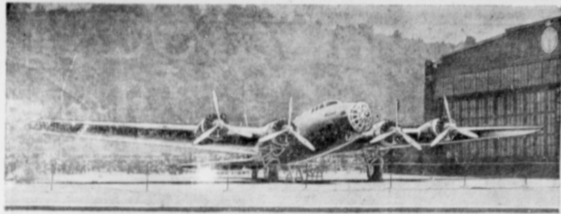
Picture of the "mystery" bomber recently completed by Boeing Airplane Company in Seattle. The ship's four motors develop 3,000 horsepower. The wing spread is 104 feet. This swift giant of the skies is expected to attain a speed of 250 miles an hour. (Photograph, Courtesy Shell Oil Company Aviation Department).
