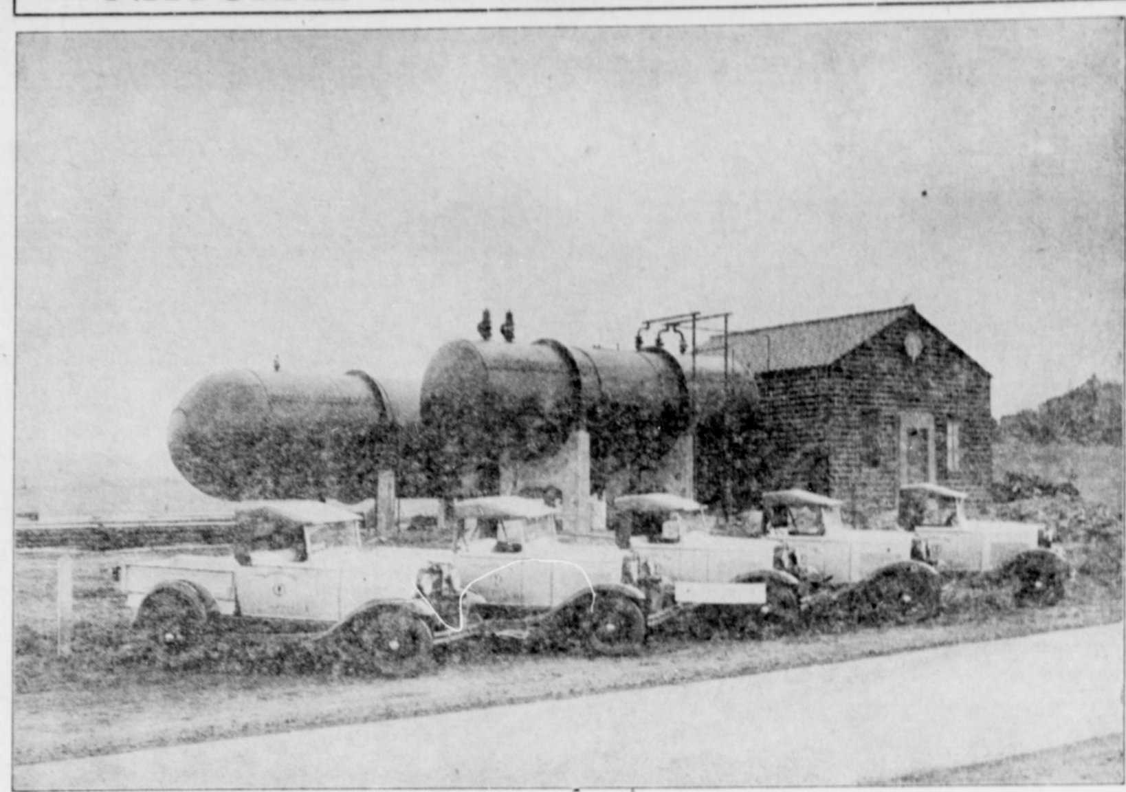
This picture shows how the plant of the Natural Gas Corporation of Oregon will look upon completion. The plant building will be approxi- mately 20x25 feet. There will be one 15,000 gallon liquid storage tank and one 12,500 cubic foot stor-
